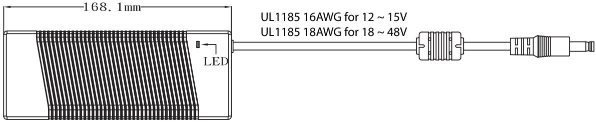
TOP-VIEW
