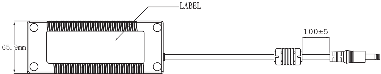
BOTTOM-VIEW
